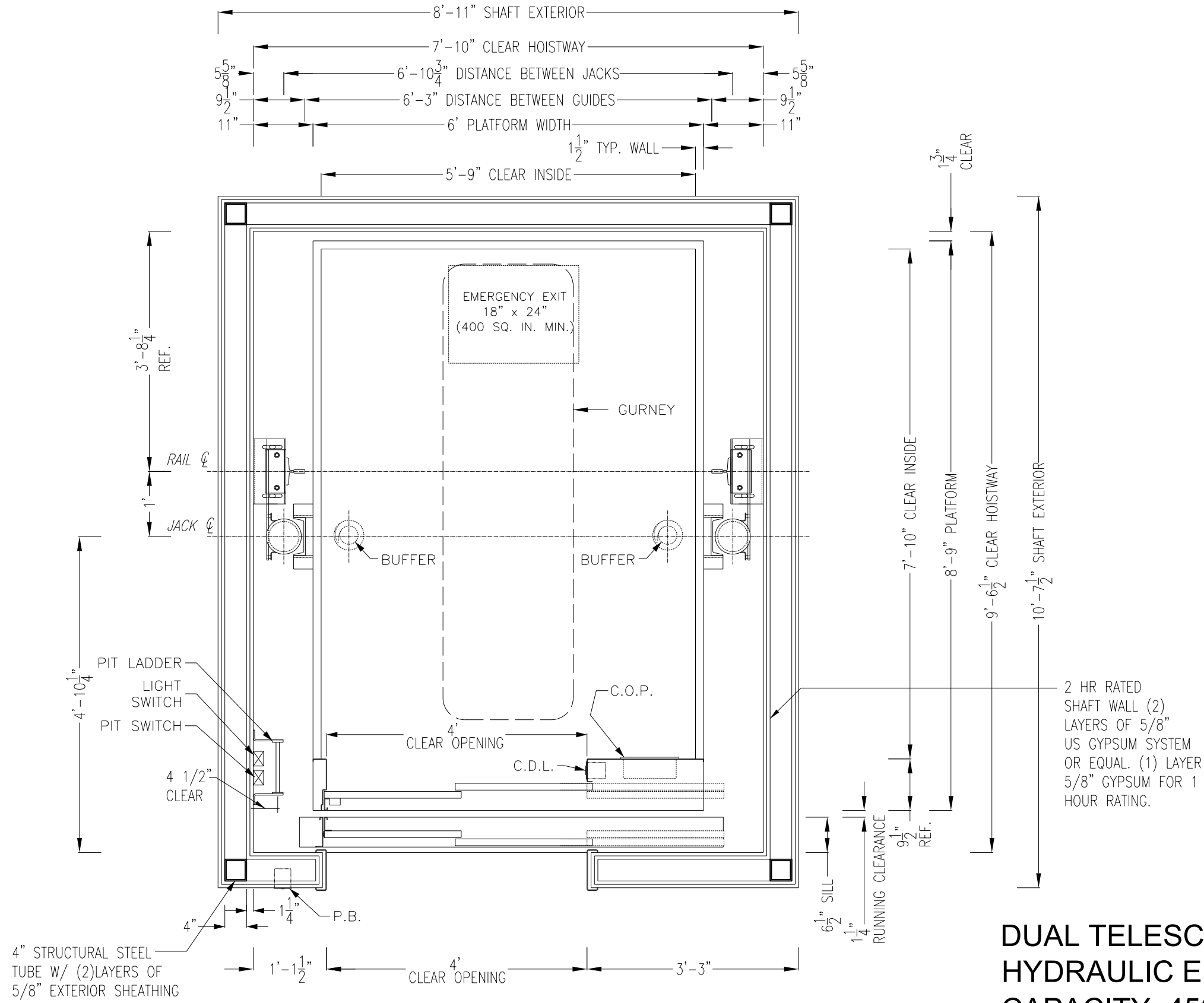
HOISTWAY PLAN
